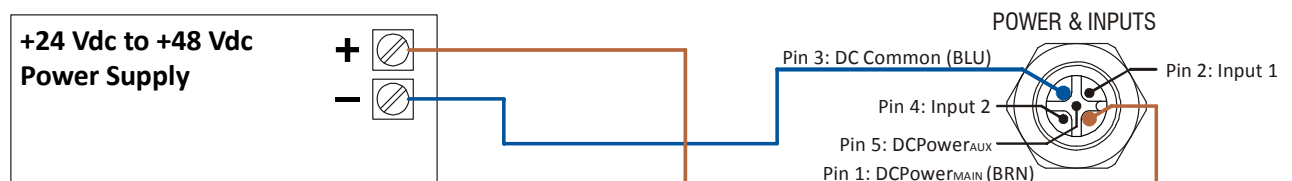
Figure T1.3 SMD17E2 Main Power Wiring
