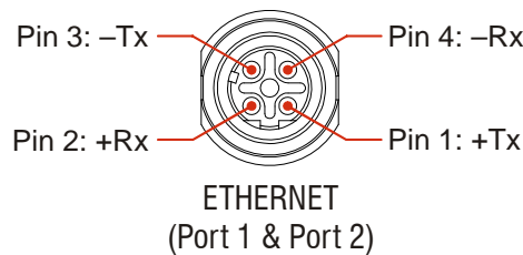
Figure R1.6 Ethernet Connector Pinout
