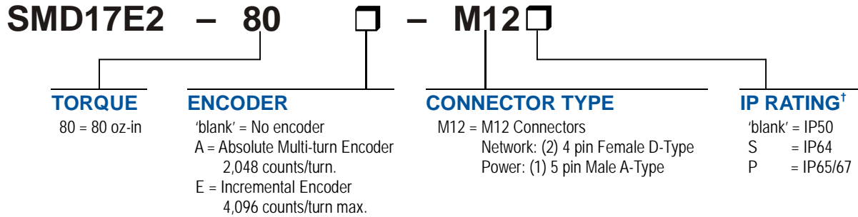
Figure R1.2 Part Numbering System
