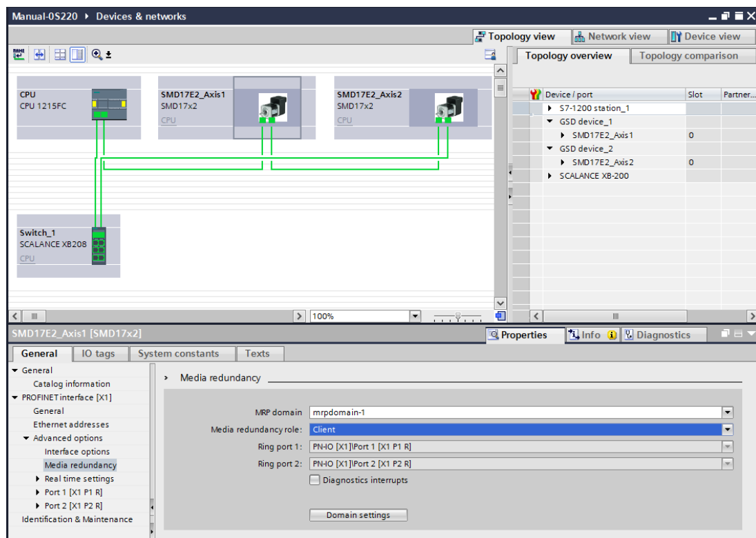
Figure T10.1 MRP Topology and Client settings
