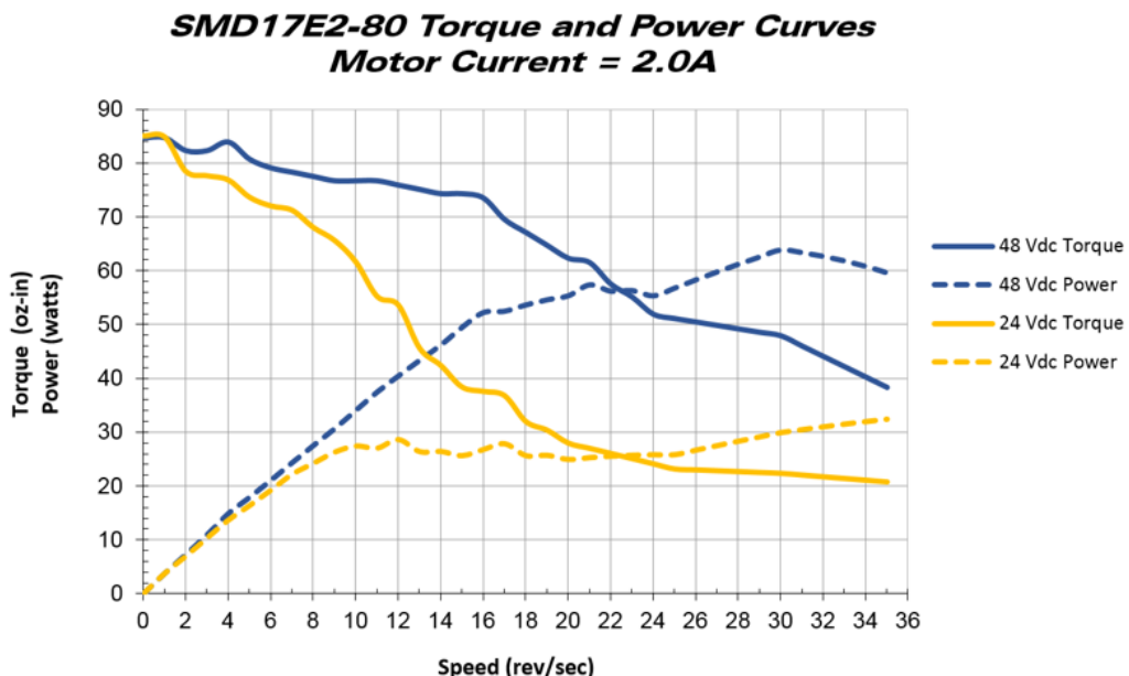
Figure R1.7 SMD17E2-80 Torque and Power Curves
