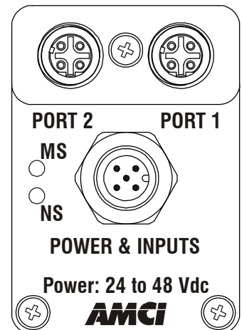
Figure R1.4 SMD17E2 Connector Locations
