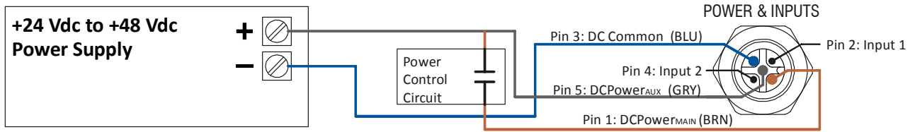
Figure T1.4 SMD17E2 Auxiliary Power, Single Supply Wiring
