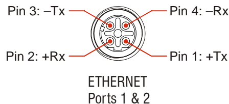
Figure T1.7 M12 Ethernet Connector Pinout
