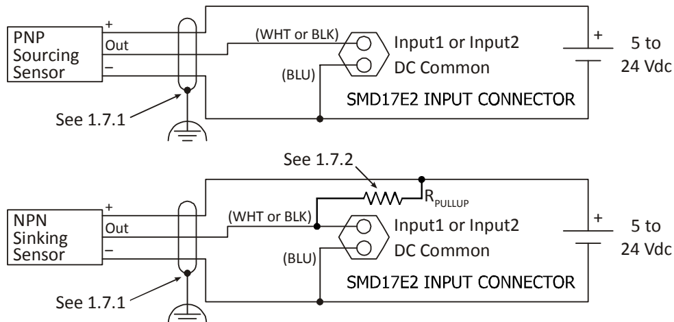
Figure T1.6 Input Wiring
