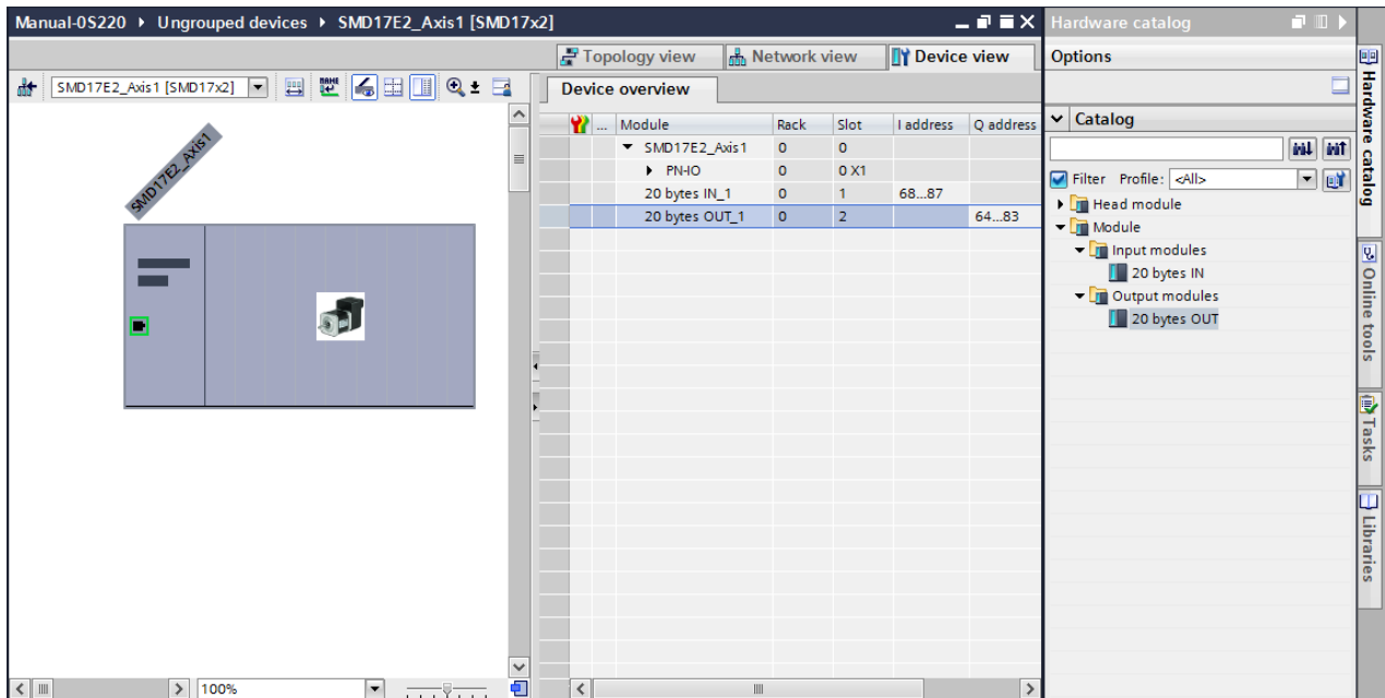
Figure 020.10 I/O Byte Mapping
