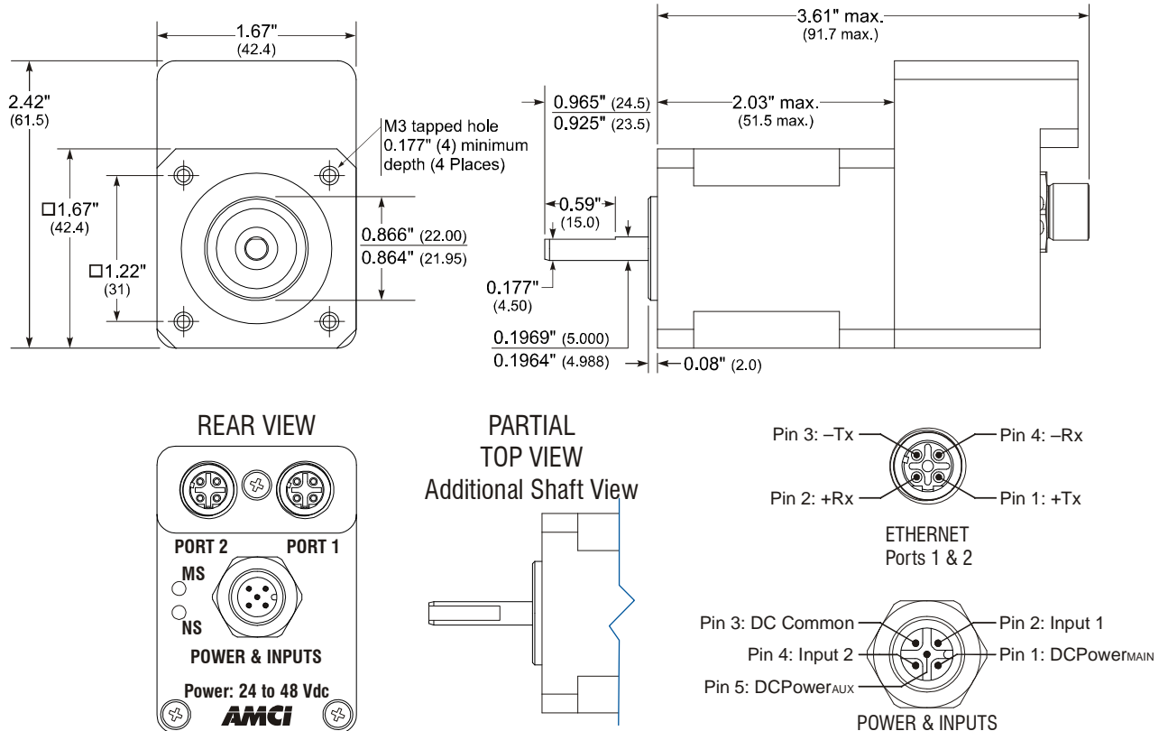
Figure T1.1 SMD17E2-80 Outline Drawing
