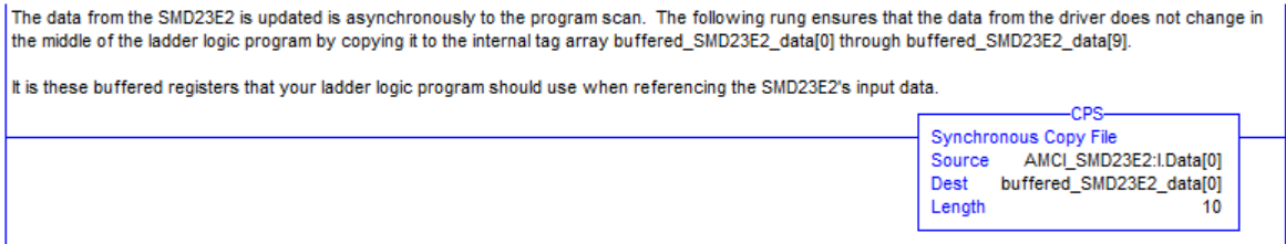
Figure T4.4 Buffer I/O Data
