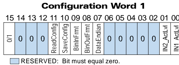
Figure R5.2 Configuration Mode: Config Word Format
