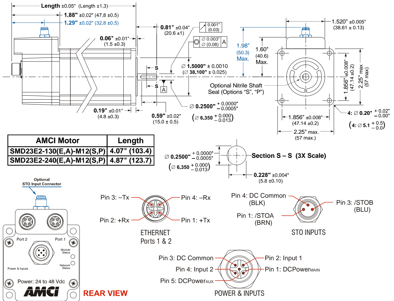
Figure T1.1 SMD23E2 Outline Drawing
