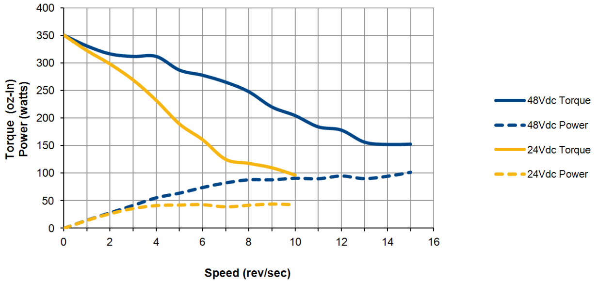
Figure R1.10 SMD24E2-350 Torque and Power Curves
