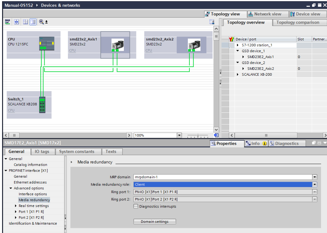
Figure T7.6 MRP Topology and Client settings
