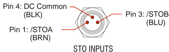
Figure T1.8 Input Wiring
