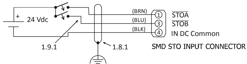
Figure T1.9 STO Input Connections
