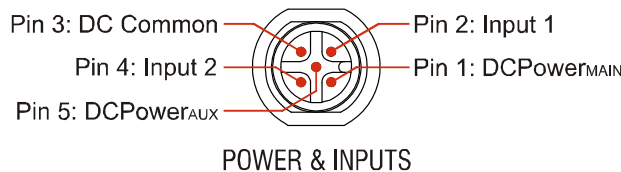
Figure R1.5 M12 Power and Inputs Connector
