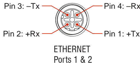
Figure R1.6 Ethernet Connector Pinout
