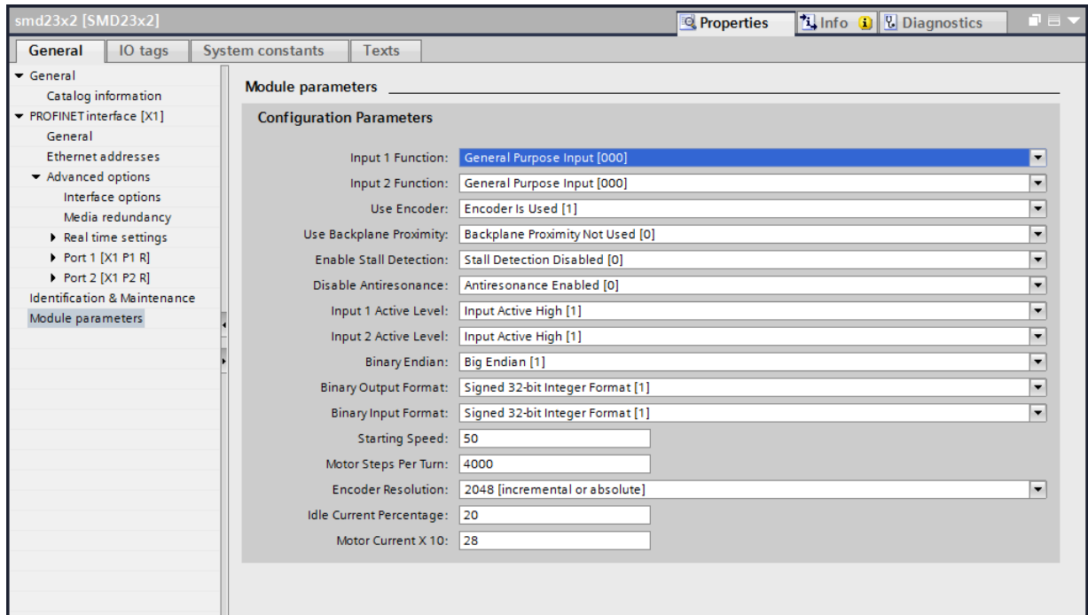
Figure T7.5 Configuration Parameters Settings
