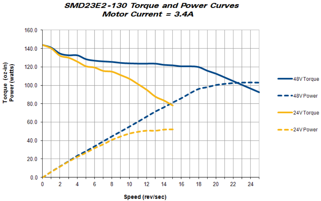
Figure R1.8 SMD23E2-130 Torque and Power Curves
