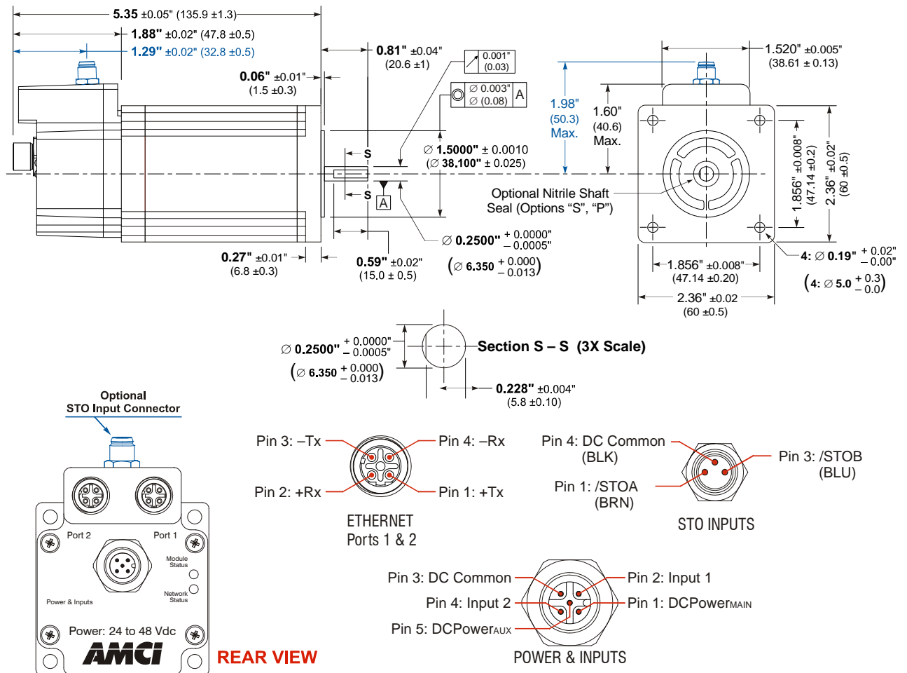
Figure T1.2 SMD24E2 Outline Drawing
