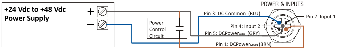
Figure T1.5 SMD23E2 and SMD24E2 Auxiliary Power, Single Supply Wiring
