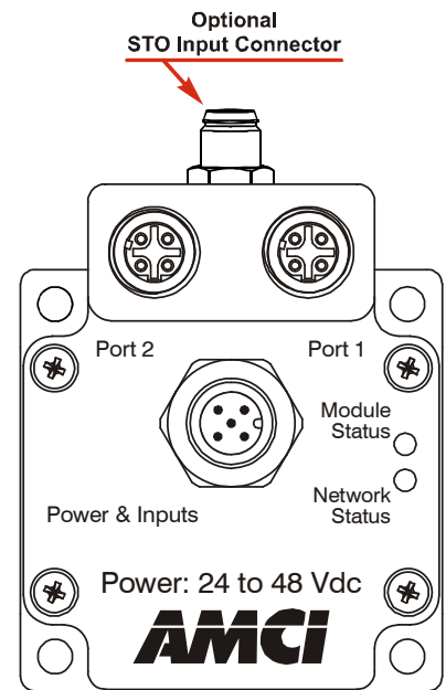
Figure R1.4 Connector Locations
