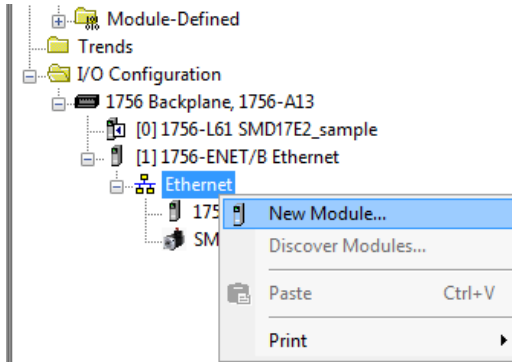
Figure T4.1 Adding an AMCI SMD23E2 or SMD24E2
