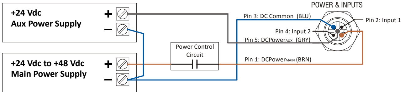
Figure T1.6 SMD23E2 and SMD24E2 Auxiliary Power, Dual Supply Wiring
