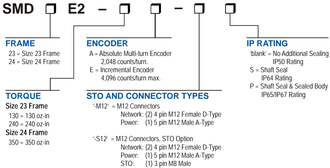
Figure R1.2 Part Numbering System
