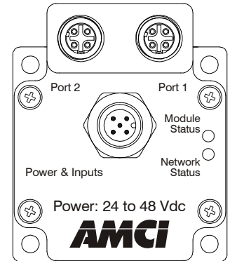
Figure R1.3 Rear Cover Status LED's
