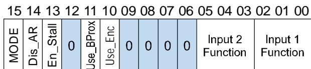
Figure R5.1 Configuration Mode: Control Word Format
