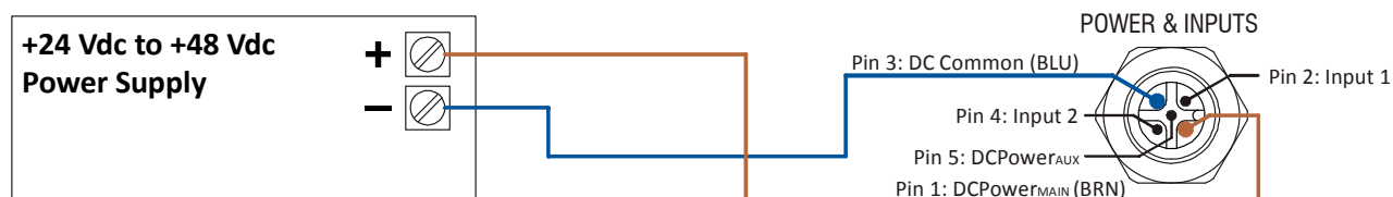
Figure T1.4 SMD23E2 and SMD24E2 Main Power Wiring
