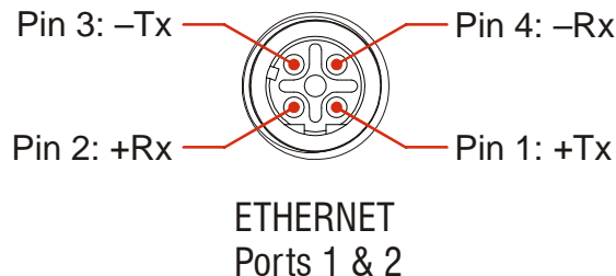
Figure T1.10 M12 Ethernet Connector Pinout
