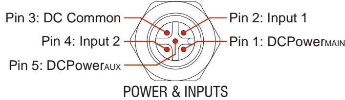
Figure T1.3 Power and Input Connector
