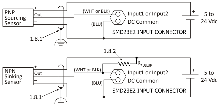
Figure T1.7 Input Wiring
