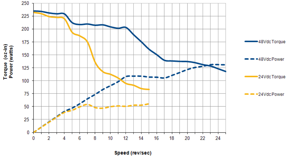
Figure R1.9 SMD23E2-240 Torque and Power Curves
