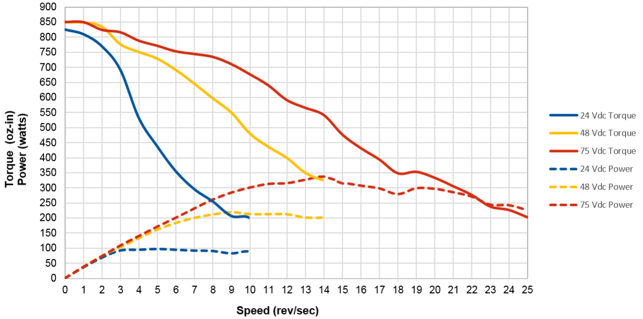
Figure R1.10 SMD34E-850 Torque and Power Curves
