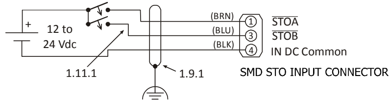
Figure T1.12 STO Input Connections
