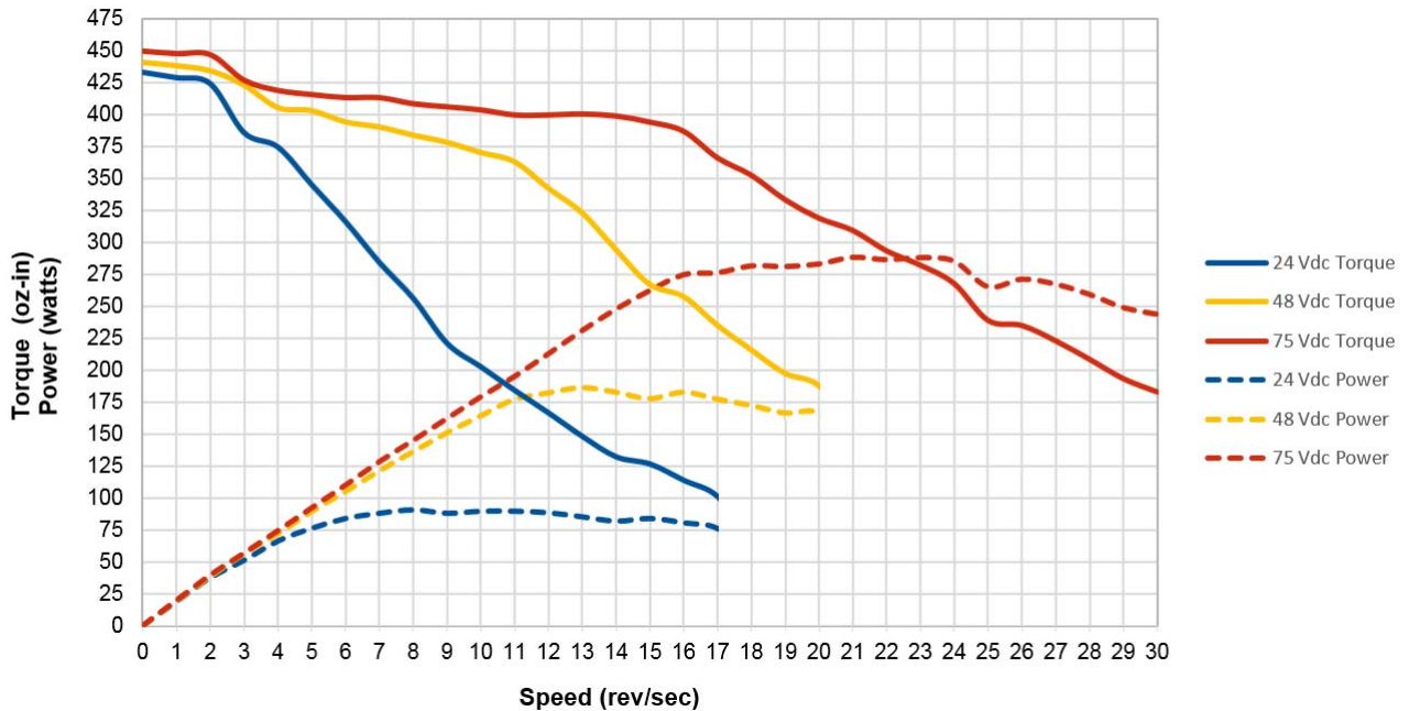
Figure R1.9 SMD34E-450 Torque and Power Curves
