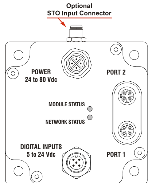
Figure R1.4 SMD34E2 Connector Locations
