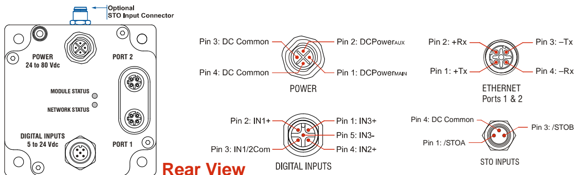
Figure T1.1 SMD34E2 Outline Drawing
