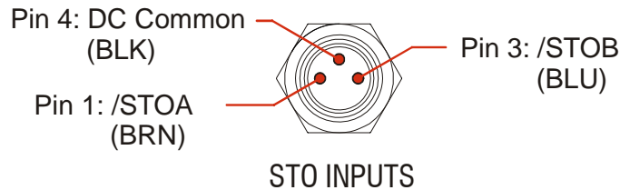
Figure T1.11 STO Input Connector
