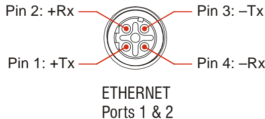
Figure T1.13 M12 Ethernet Connector Pinout
