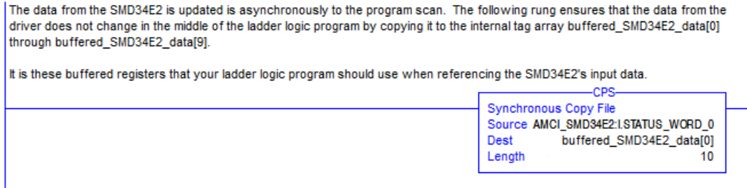
Figure T4.4 Buffer I/O Data
