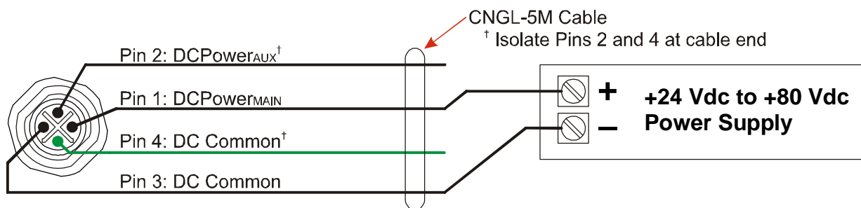
Figure T1.3 SMD34E2 Main Power Wiring
