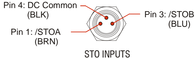
Figure R1.8 STO Connector Pinout
