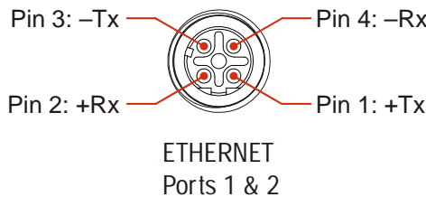
Figure R1.6 Ethernet Connector Pinout
